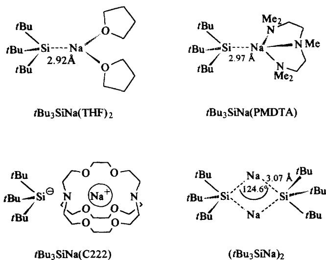
Fig. 2. Structures of t\text{Bu}_3\text{SiNa}(\text{THF})_2 (X-ray; H. Nöth, I. Krossing), t\text{Bu}_3\text{SiNa}(\text{PMDTA}) (X-ray; H. Nöth, M. Schmidt-Amelunxen), t\text{Bu}_3\text{SiNa}(\text{C222}) (assumption) and (t\text{Bu}_3\text{SiNa})_2 (X-ray; H. Nöth, M. Schmidt-Amelunxen).
